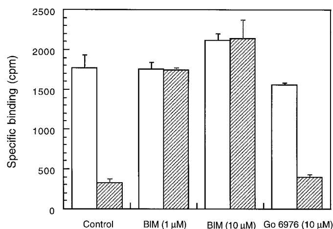
Fig. 7. Effects of PKC inhibitors on down-regulation of TNF receptors by PDBu. Cells were pretreated with or without 1.0 \mu M BIM, 10 \mu M BIM, or 10 \mu M Gö 6976 for 1 hr and then treated with or without 1.0 \mu M PDBu for 1 hr. Specific binding of ^{125} I-TNF was determined as described in Experimental Procedures. □, -PDBu; ▨, +PDBu. Results are means of two to three independent experiments performed in duplicate. Bars, mean \pm standard error.
