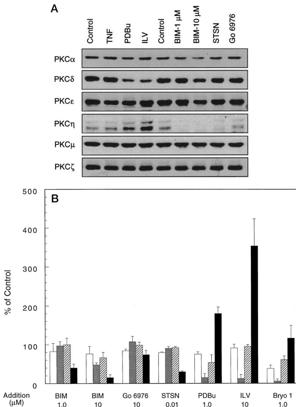
Fig. 5. Effects of PKC modulators on the expression of PKC isozymes in MCF-7 cells. A, MCF-7 cells were treated with or without 1.0 nM TNF, 1.0 \mu M PDBu, 10 \mu M ILV, 1.0 \mu M BIM, 10 \mu M BIM, 10 nM staurosporine (STSN), or 10 \mu M Gö 6976 for 6 hr as indicated. Western blot analyses were performed with total cellular extracts using PKC isozyme-specific antibodies. The same blot was probed with different antibodies. Results are representative of three to five experiments. B, The abundance of PKC isozymes was quantified by scanning immunoblots with a laser densitometer, and the values are the means \pm standard error of three to five individual experiments. \square , PKC \alpha ; \blacksquare , PKC \delta ; \hline , PKC \epsilon ; and \blacksquare , PKC \eta .
