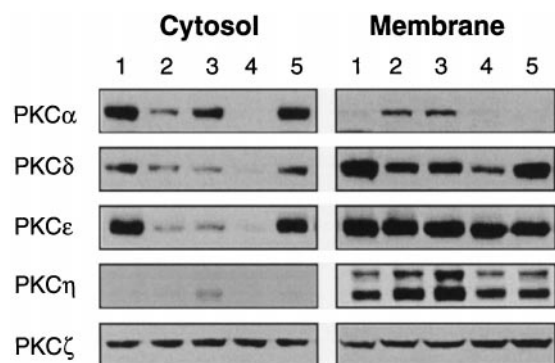
Fig. 6. Effects of TNF and PKC activators on the subcellular distribution of PKC isozymes. Cells were incubated without (lane 1) or with 1.0 \mu M PDBu (lane 2), 10 \mu M ILV (lane 3), 1.0 \mu M bryostatin 1 (lane 4), or 1.0 nM TNF (lane 5) for 6 hr. Cytosol and membrane fractions were separated, and Western blot analyses were performed with PKC isozyme-specific antibodies.
